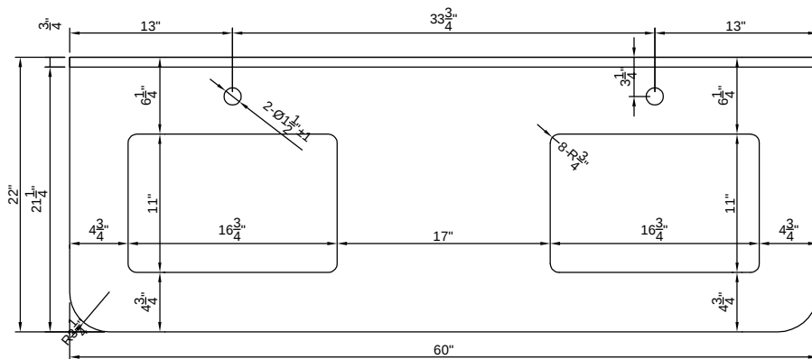
TOP VIEW OF VANITY CABINET
