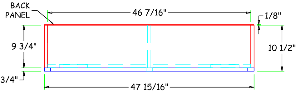
< PLAN VIEW >
