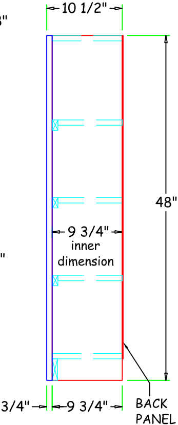
< SIDE VIEW >
