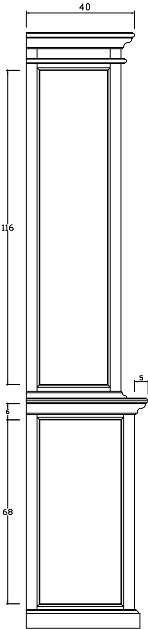
SIDE VIEW
