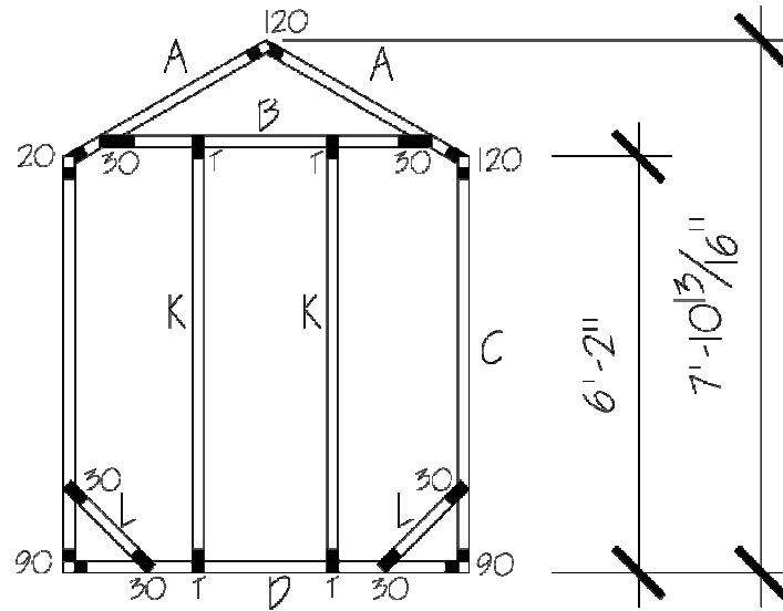
REAR ELEVATION
