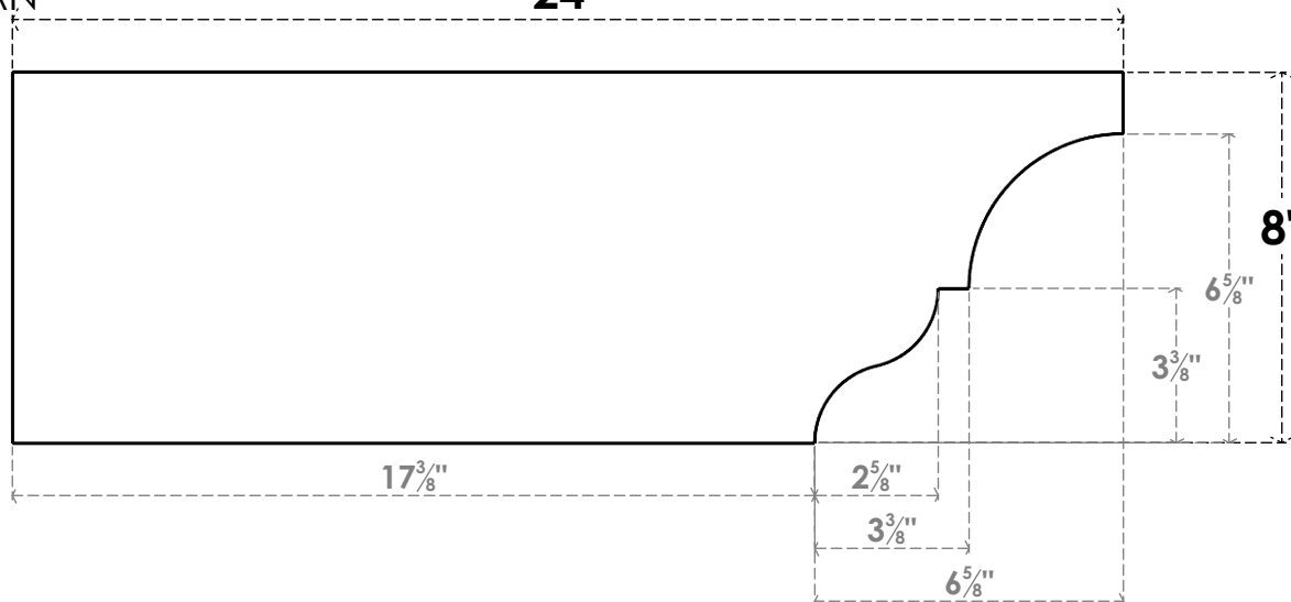
SIDE PROFILE
