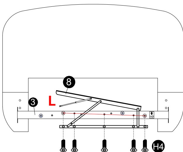
Headboard fixing holes position
