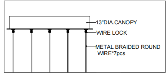
CANOPY DETAIL
