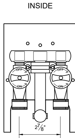
OPEN SIDE VIEW
