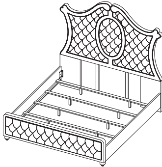
COMPLETED KING BED ASSEMBLY
