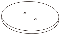
B-240X240X12mm(1pc)
