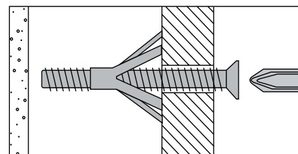
3. Cavity Fixing Wall Plug
