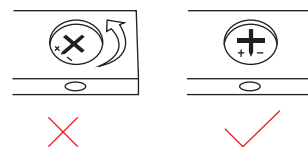
6. Pay attention to aligning the eccentric part with the screw rod
