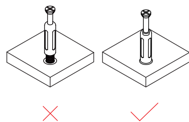
3. Pay attention to tightening the screw rod
