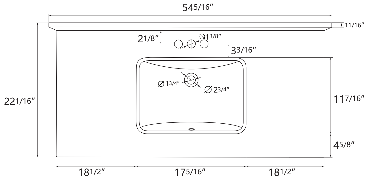
Top View
