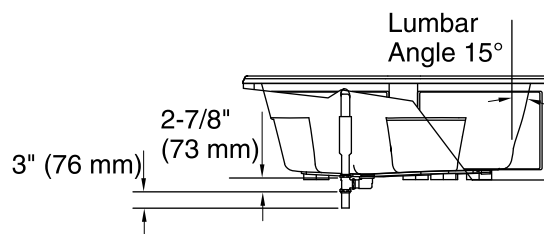
Drop-In Rim Style Cut-Out Detail
