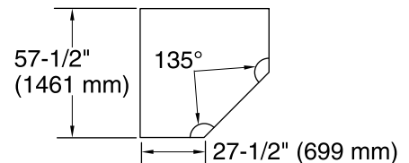
Drop-In Rim Style Cut-Out Detail
