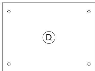
BA1846 514x382x38mm
