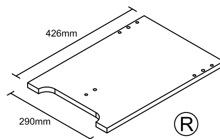
STOOL SIDE PANEL
