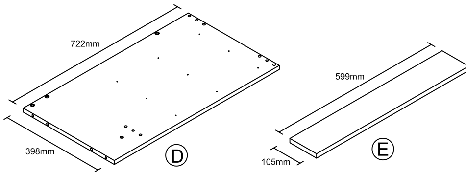
PARTITION PANEL
