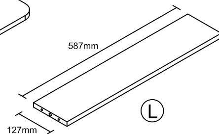
RAIL
