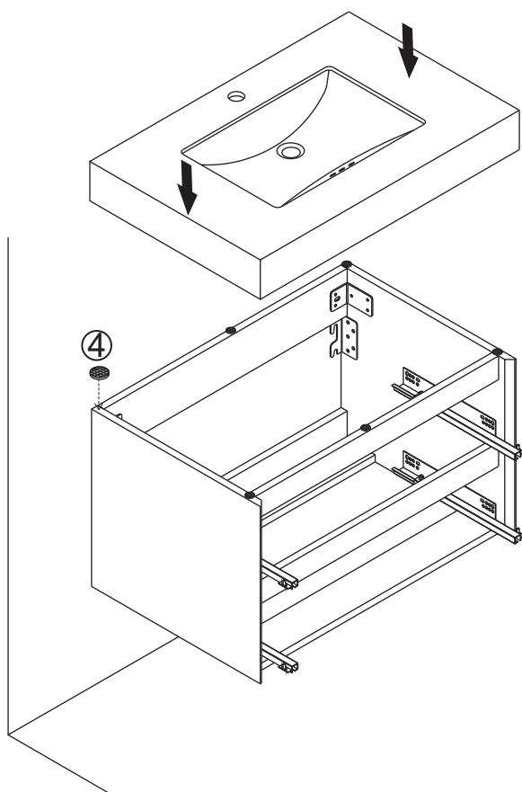
Installation of drain assembly
