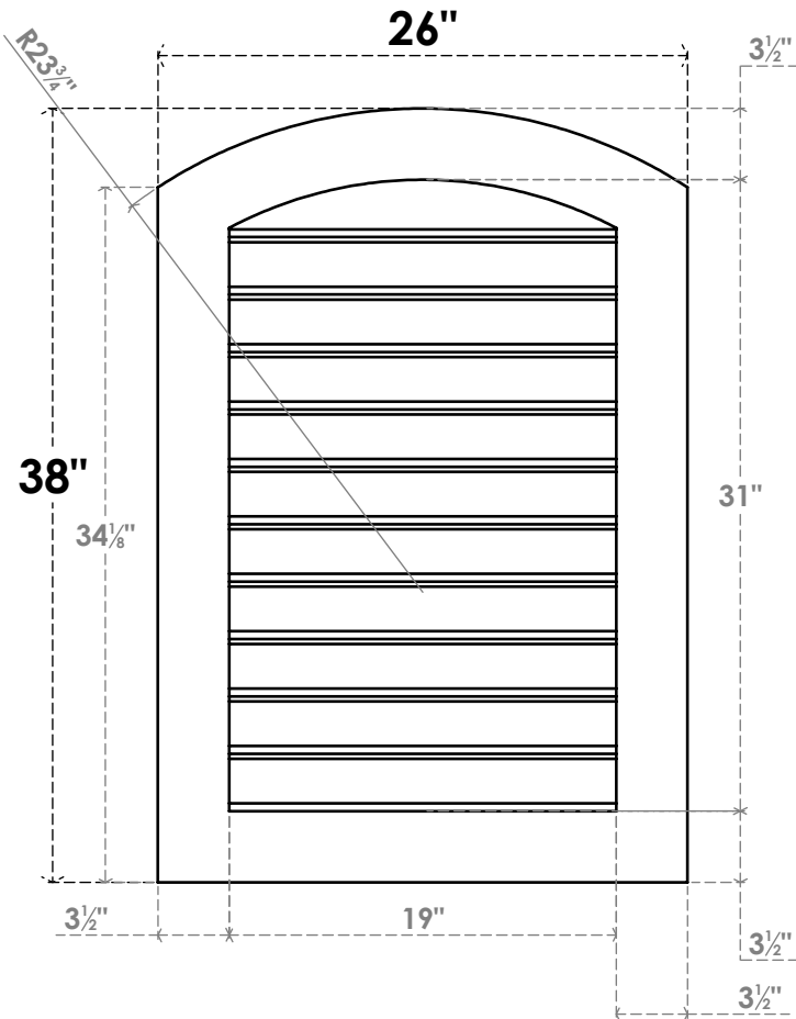
FRONT
