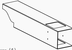
Post Arm (1) 5" x 5" x 25½"
