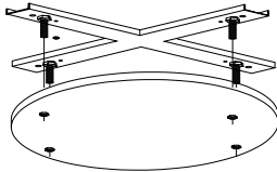
4. Mounting bracket for fixing lamp
