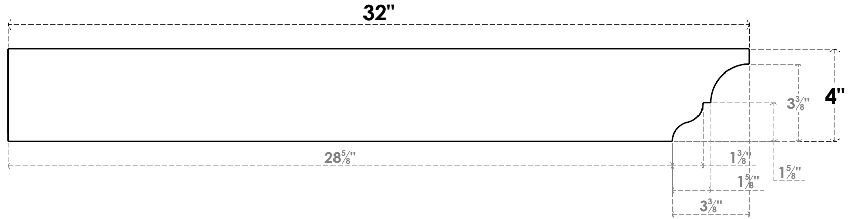
SIDE PROFILE
