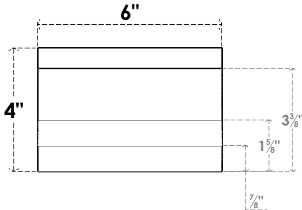
FRONT PROFILE
