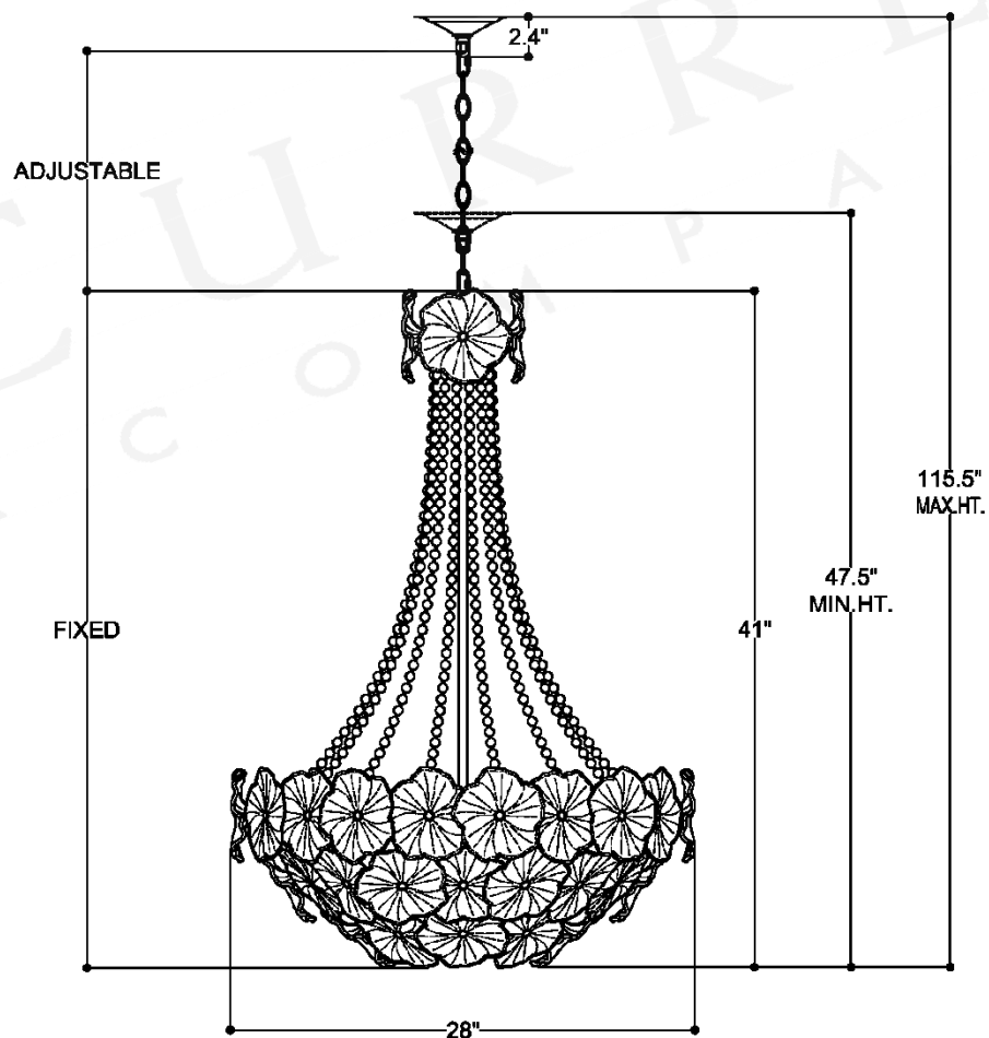
FRONT VIEW
