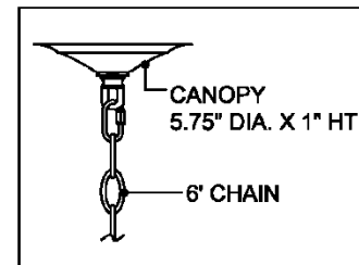
CANOPY DETAIL
