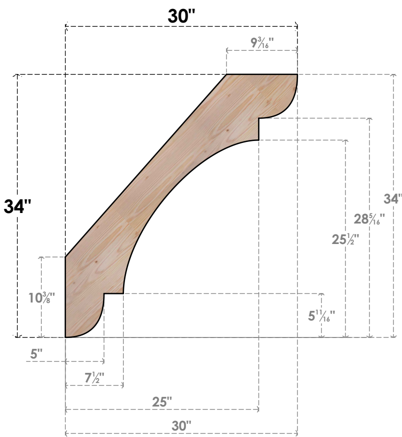
SIDE
