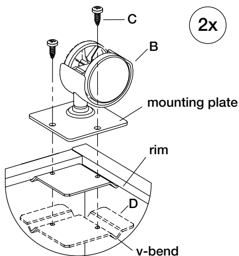
FIGURE 4: Close-up of rear caster assembly.
