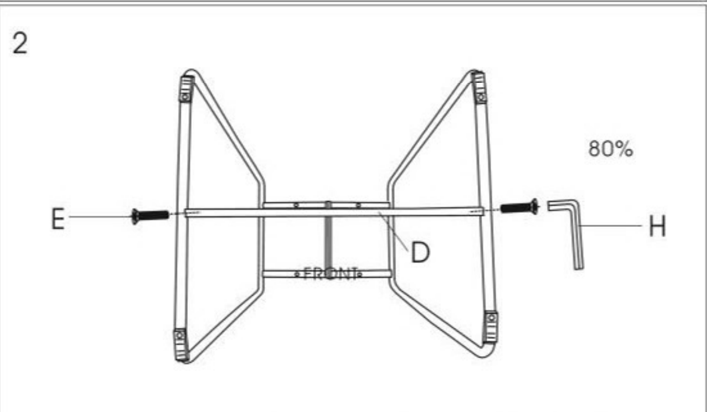
Step2: Lock the screw 80% at first.
