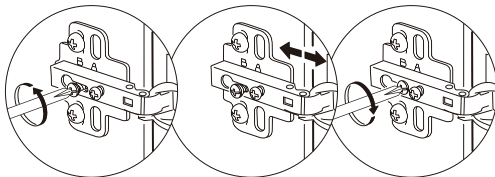
Hinge Depth Adjustment (In/Out)
