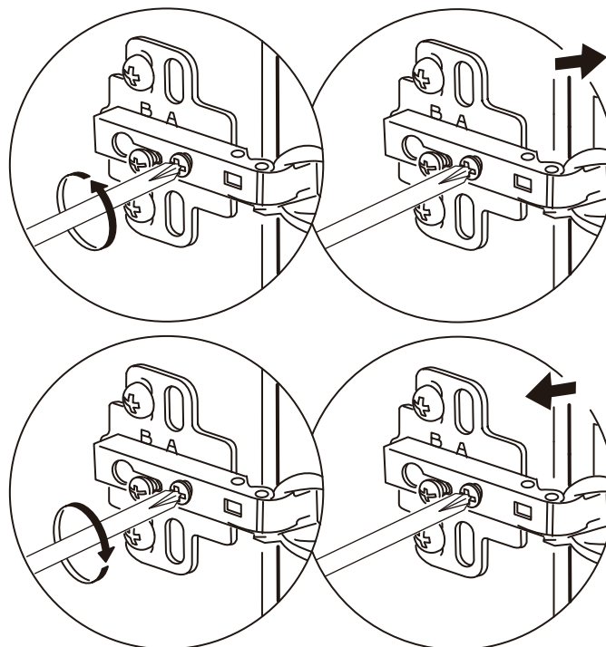
Hinge Lateral Adjustment (Left/Right)
