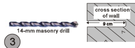
Drawing 3: Use 14-mm masonry drill to drill 9 cm deep holes.
