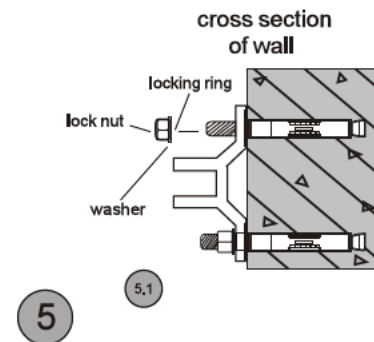
Drawing 5: Bracket has been prepared to be fixed on a wall (5.1)
