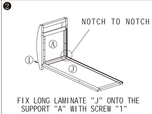
LONG LAMINATE J*1
