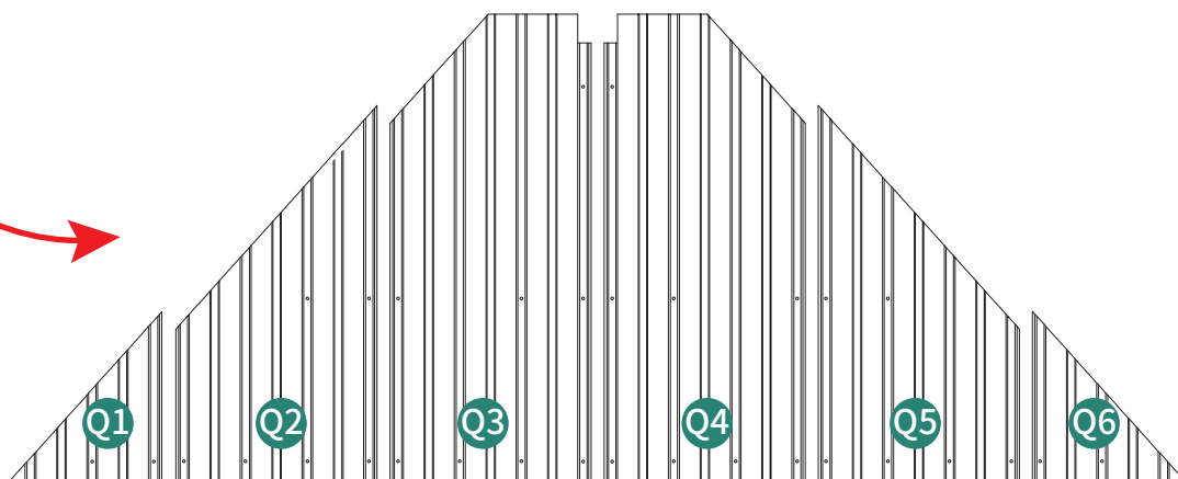
Guidelines for Roof Tile Distribution.
