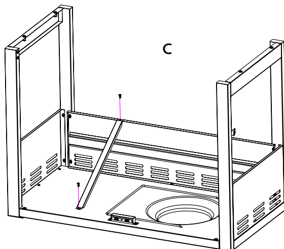
M4x10 Screw Qty: 7 pcs
