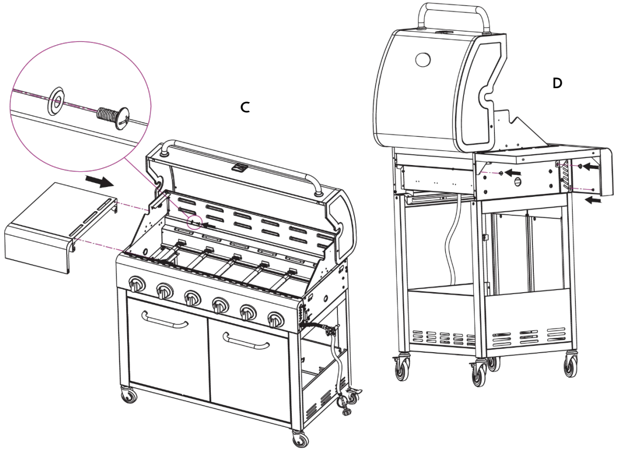
M6 Compression Washer Qty: 2 pcs
