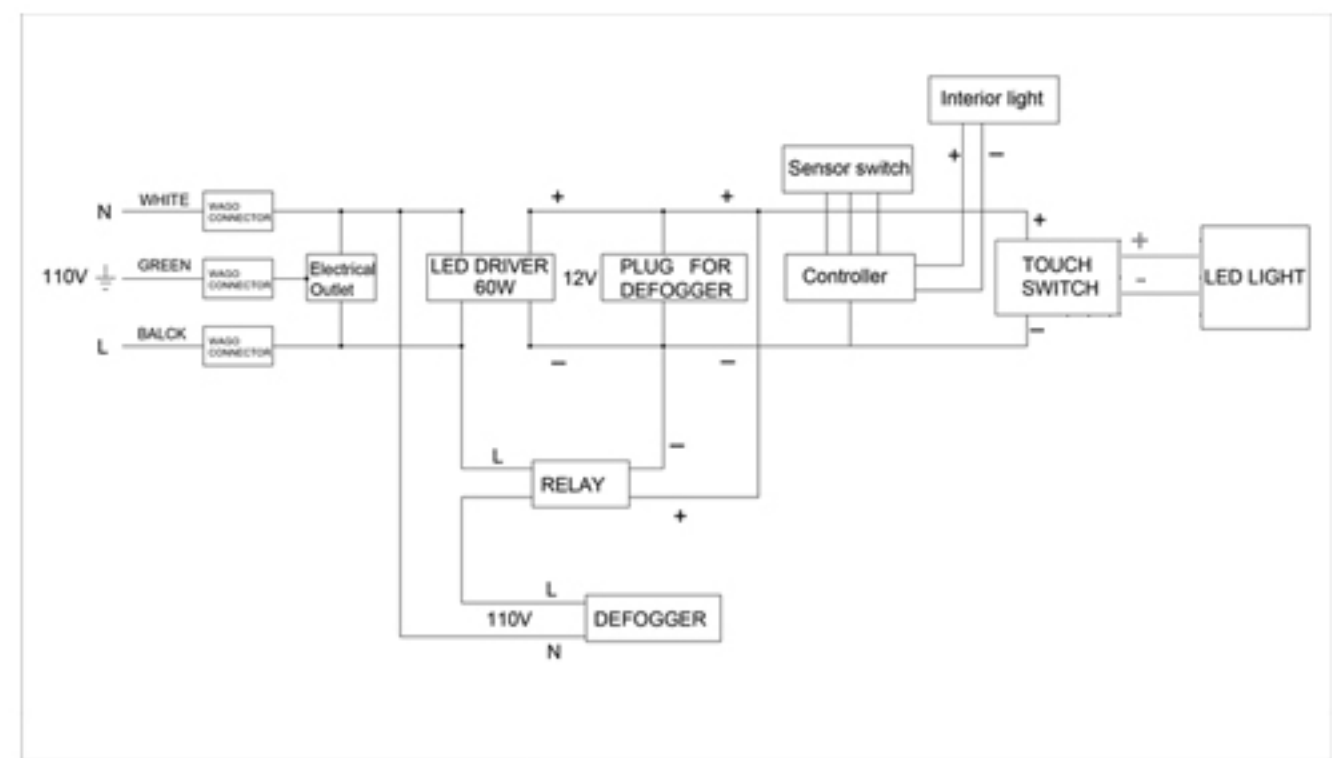
Circuit Diagram
