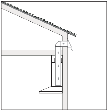
WALL EXHAUST
