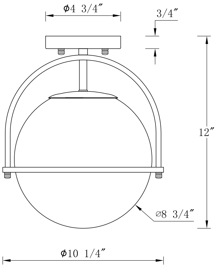
FRONT VIEW
