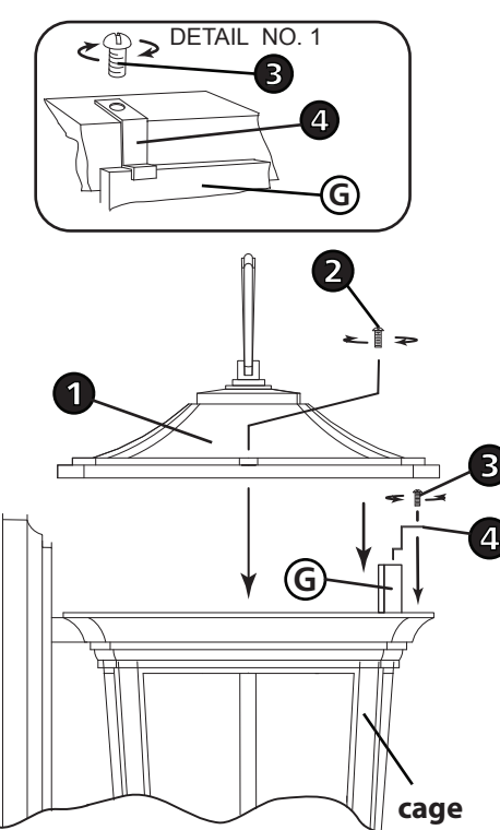
Drawing 2 – Glass Installation
