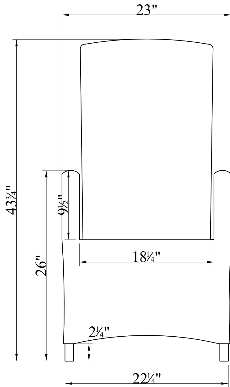
FRONT VIEW
