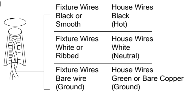
Fig.2 wiring
