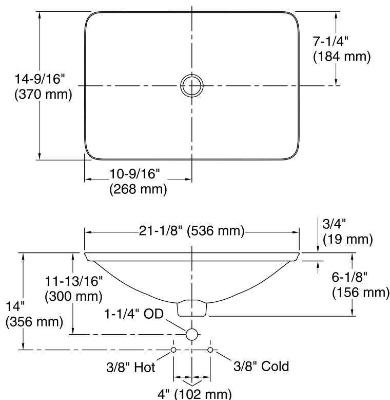
Standard Installation
