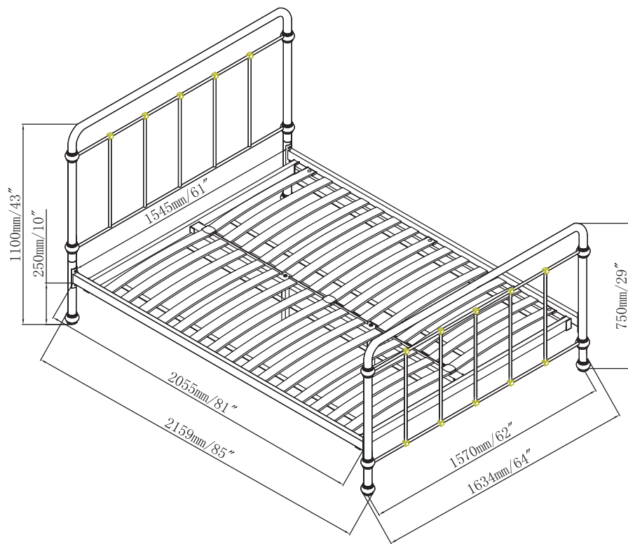
Product Dimension
