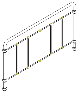
③ Footboard 1634x64x750mm (1)
