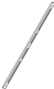
⑥ Center Rail 25x50x1885mm (1)
