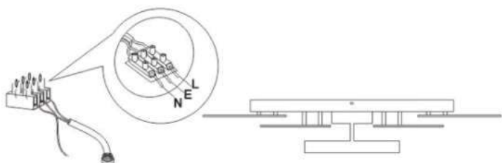
3. Connect the power supply, and align the hole position on the lamp base with the hole position on the cross.
