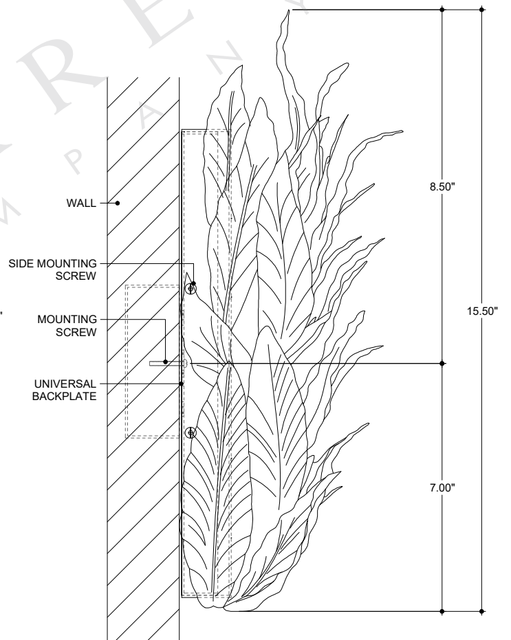
SIDE VIEW
