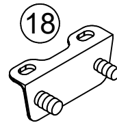
x4 #A54203 drawer bracket
