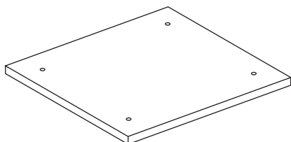
A 435*335*12mm(1pc)
