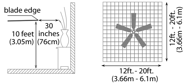
downrod installation
