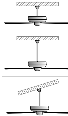
downrod installation
