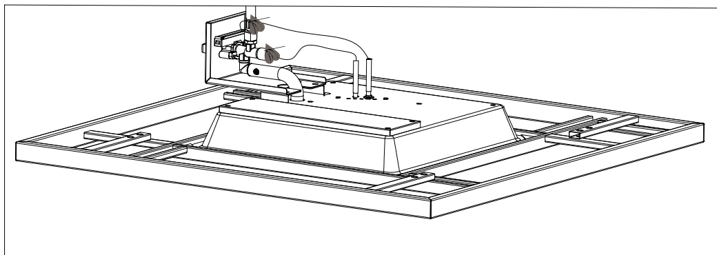
Regulator/Cylinder Connection
