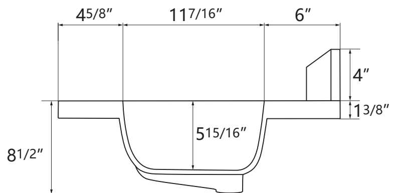
Side View
