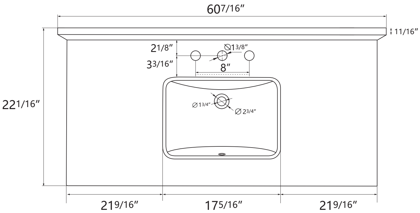
Top View
