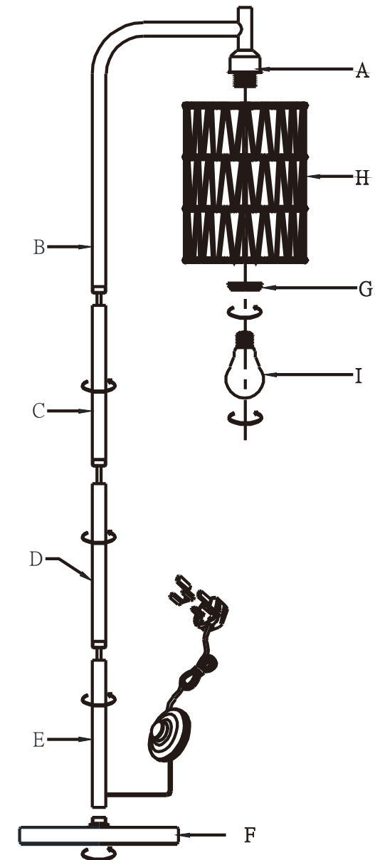
DIAGRAM 1: LAMP ASSEMBLY
