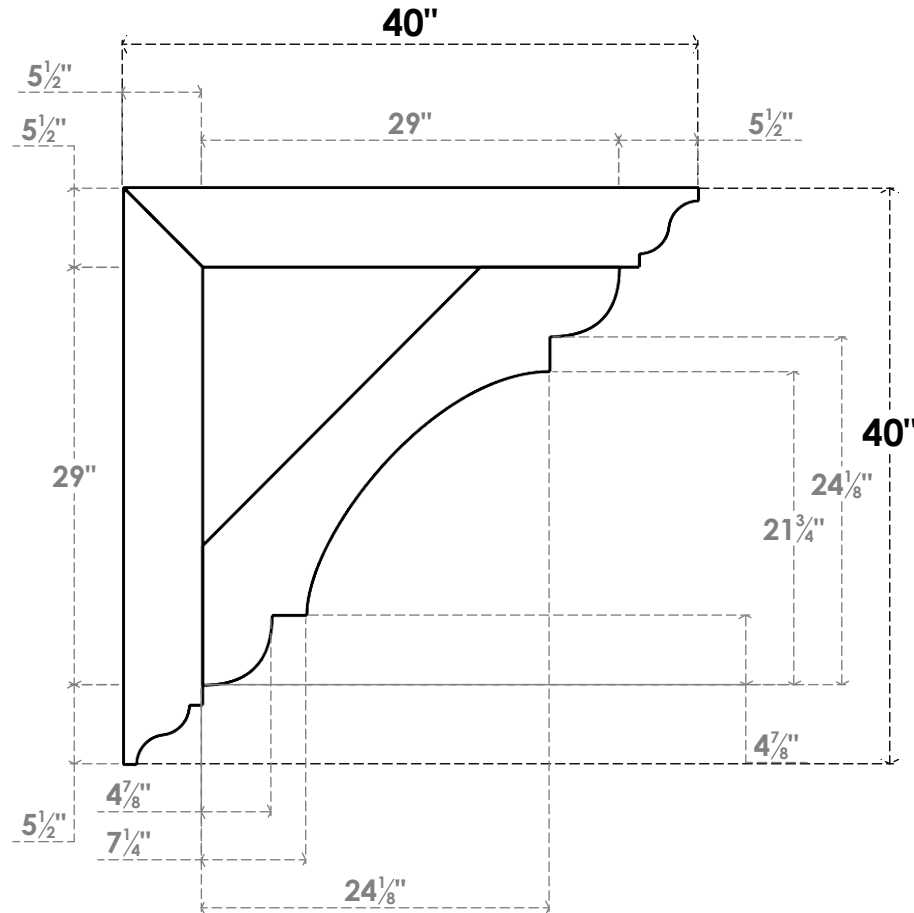
SIDE PROFILE
