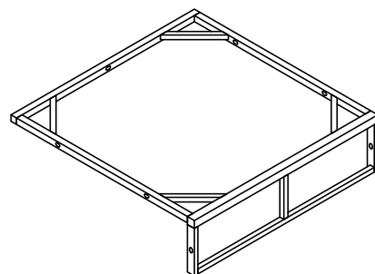
Seat frame (2 pcs)
