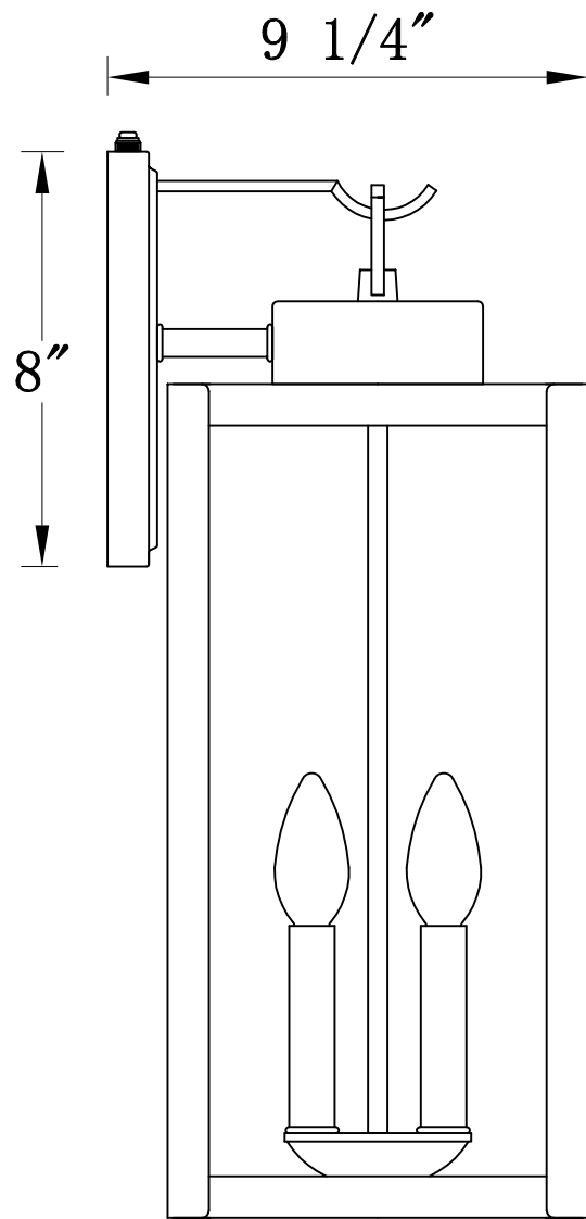
SIDE VIEW
