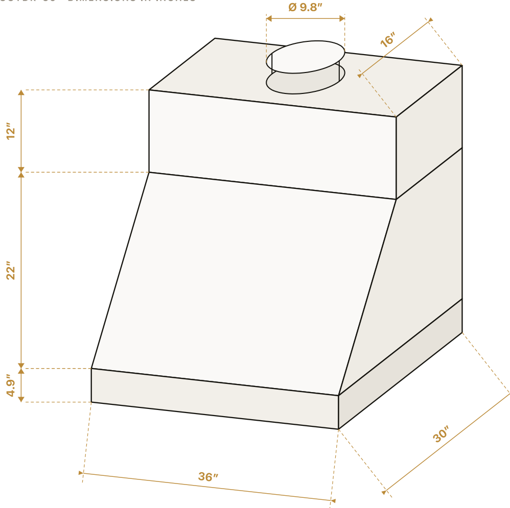
RH-OUTDR-36 · DIMENSIONS IN INCHES
